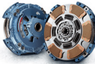
Eaton Clutch Kit Advantage@ Easy Pedal Clutch 2" 10-Spline 2050 lb-ft 308935529
