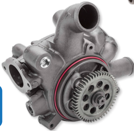
HG64 Side Inlet R23538636
